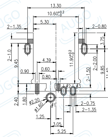
PCB LAYOUT TOP VIEW TOLERANCES:±0.05
