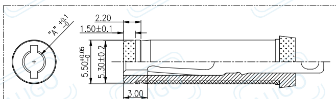
MATING PLUG
