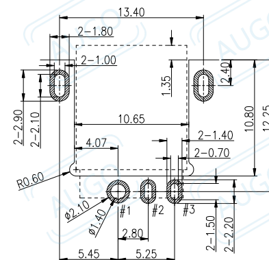
PCB LAYOUT TOP VIEW TOLERANCES:±0.05
